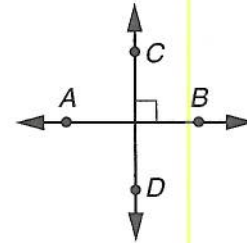
Perpendicular lines
